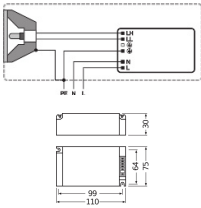
Specifications Osram PTi 1x70/220-240 S
